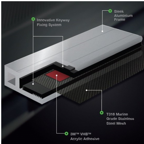
Innovative Keyway Fixing System
